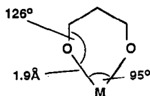
six membered
