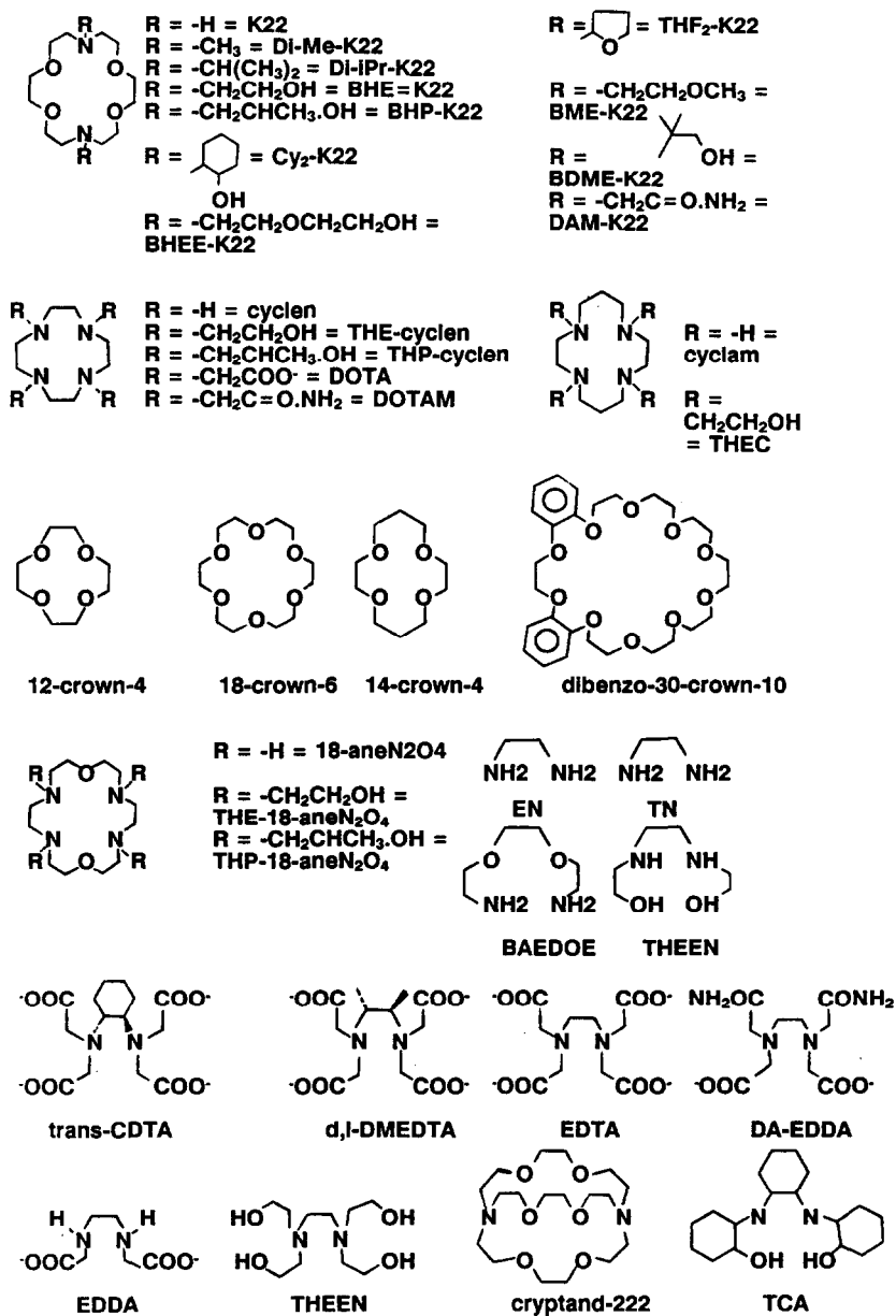
Fig. 2. Ligands discussed in this review.
