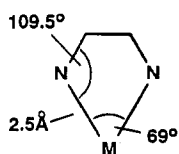
five membered
