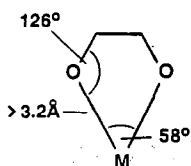
five membered
