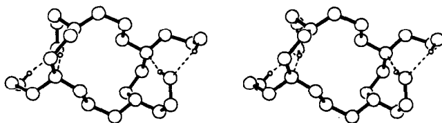
Fig. 6. Stereoview of the free ligand THEC, showing the internal hydrogen bonding (---) structure that promotes crystallinity. Redrawn using coordinates in Ref. [31].
