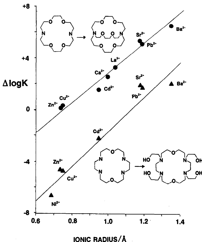
Fig. 7. Change in complex stability, \Delta \log K , that occurs on adding neutral oxygen donors to ligands, as a function of metal ion size. The upper curve (● points) shows the change that occurs on passing from K-22 to cryptand-222; the lower curve (▲ points) shows the change from 18-aneN 4 O 2 to THE-18-aneN 4 O 2 . Formation constants from Refs. [27,33].
