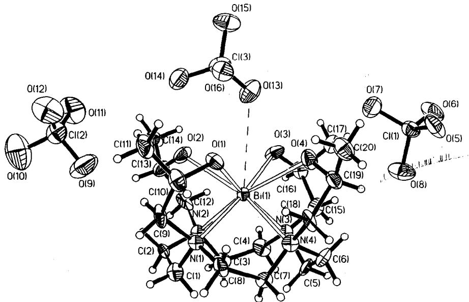
Fig. 18. Structure [61] of the Bi(III) complex of THP-cyclen, showing the suggested position of the stereochemically active lone pair, and its long bond to the perchlorate oxygen placed directly above the gap in the coordination geometry that corresponds to the position of the lone pair.
