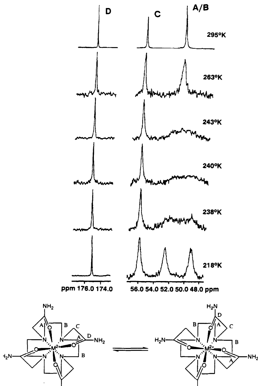
Fig. 19. (Above) ^{13}\text{C} NMR spectra [62] of the complex of Zn(II) with DOTAM at different temperatures in \text{D}_7 -DMF solution. (Below) Diagram of the Zn(II) DOTAM complex showing the assignment of the peaks in the ^{13}\text{C} NMR spectra.
