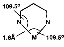
six membered
